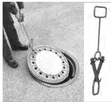
Universal hand grips with hook
