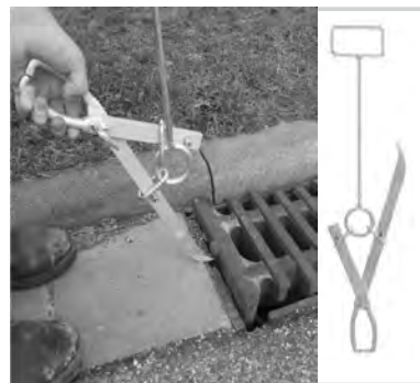
Universal hand grips with hook and break-away lever
